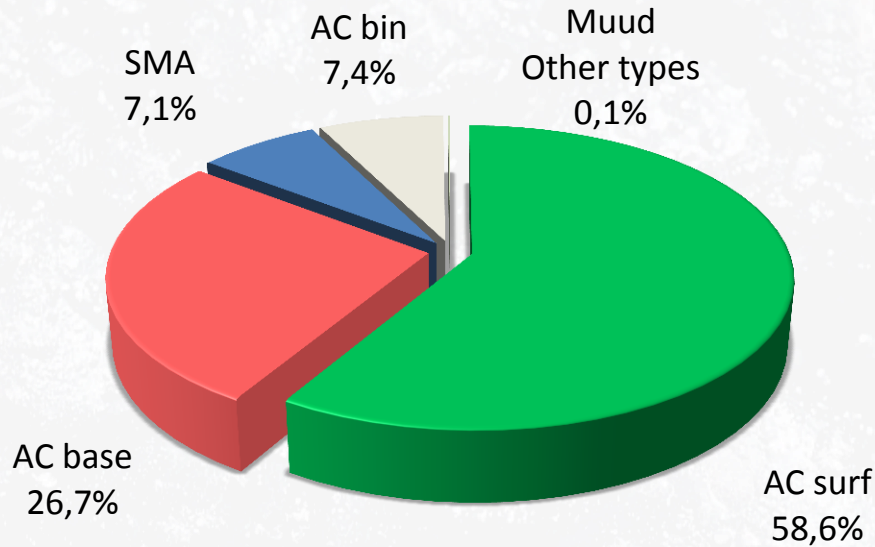
TOODETUD ASFALTSEGUSID Produced Asphalt Mixtures
